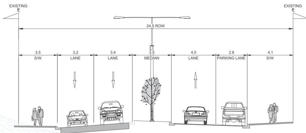
Cross section view from this point looking north
