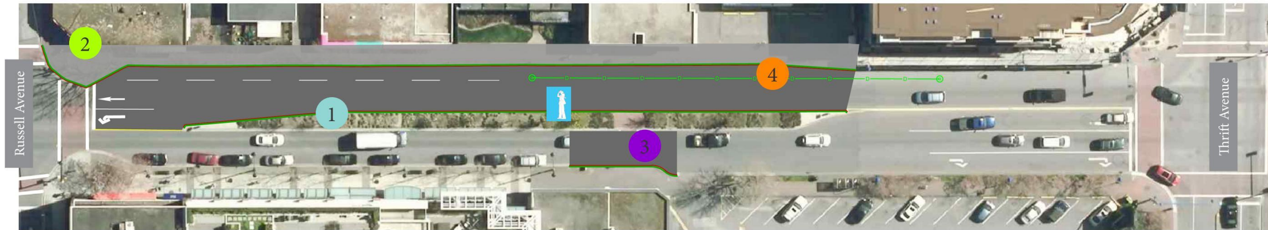
1 Median planting to prevent illegal crossing
