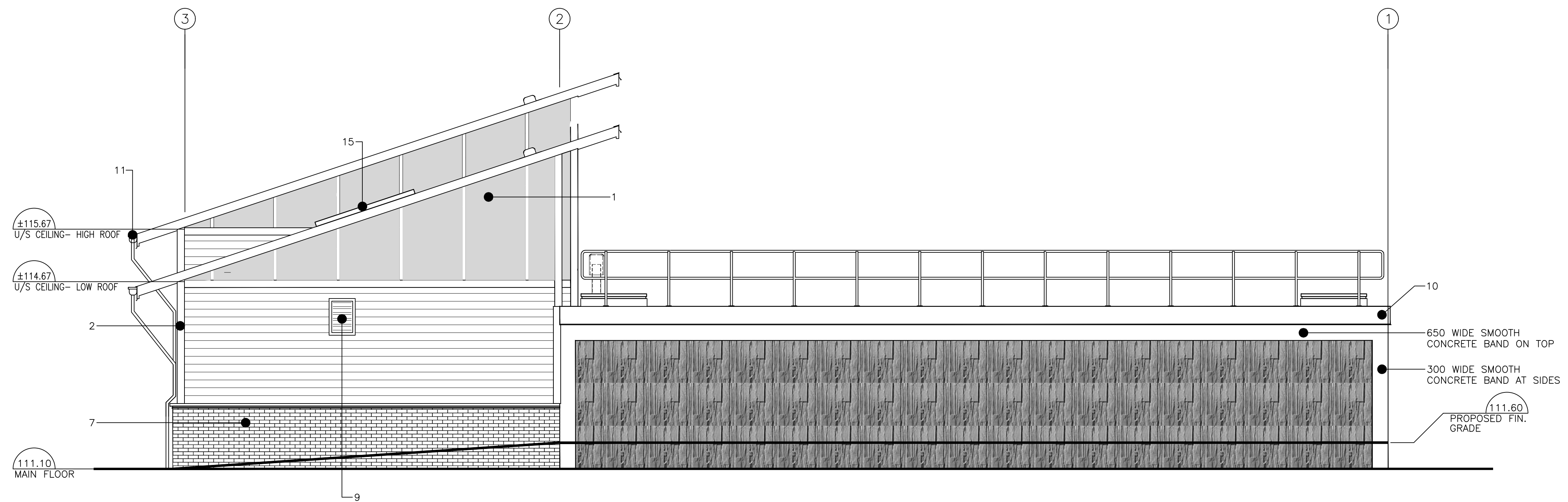
NORTH ELEVATION SCALE 1:50
