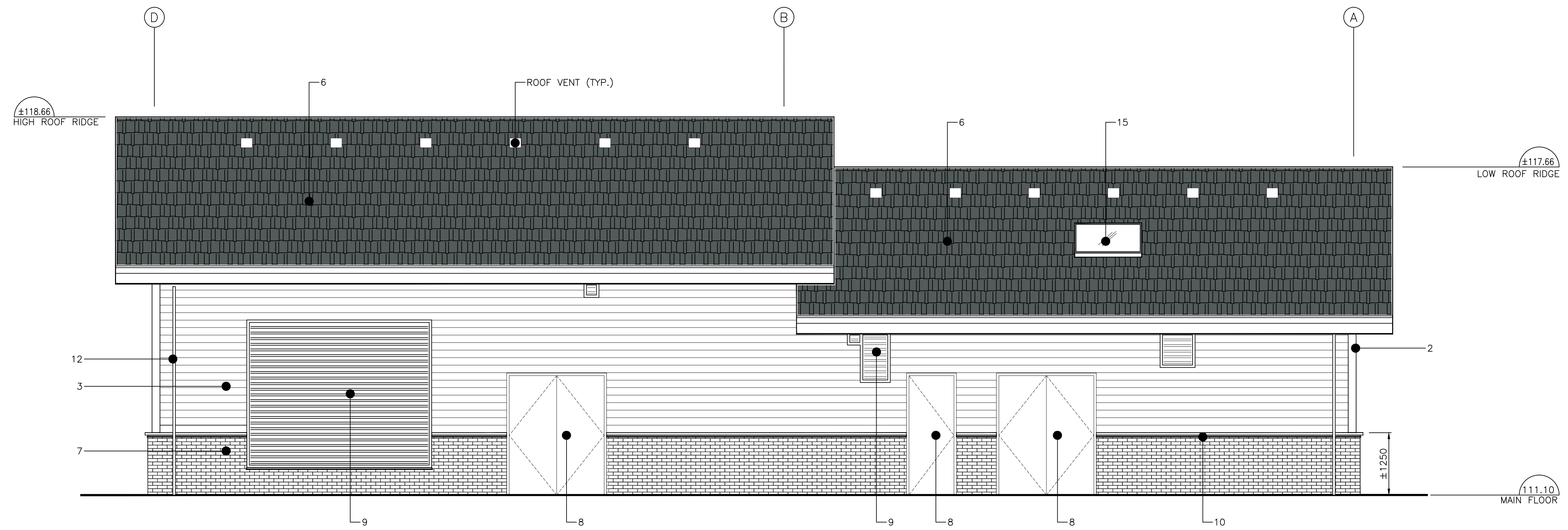
EAST ELEVATION SCALE 1:50
